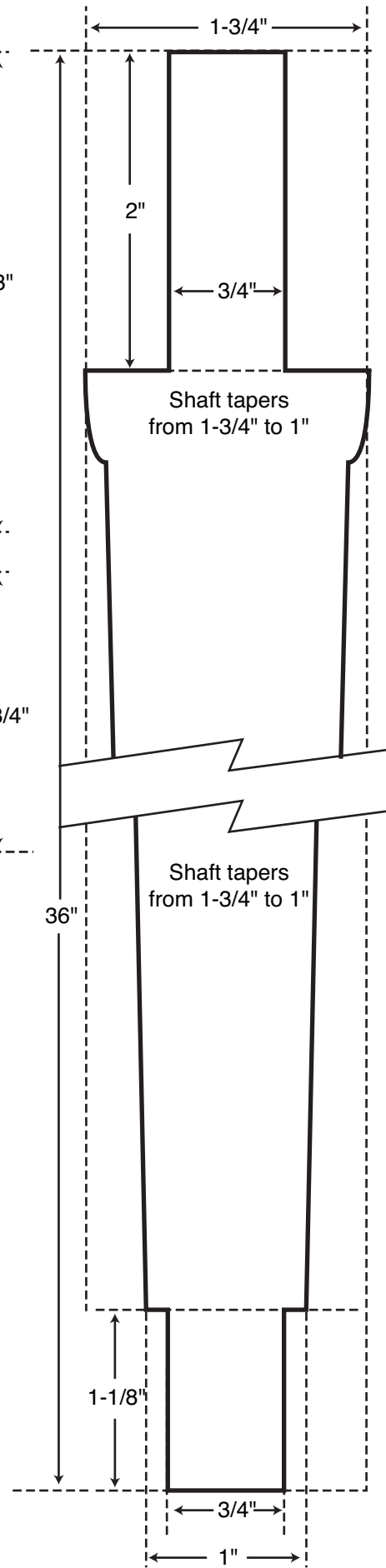
Cane Shaft Dimensions
